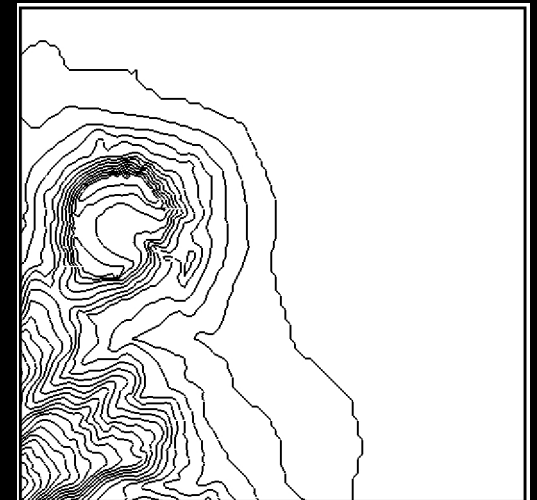
Contour plot of Honolulu data
