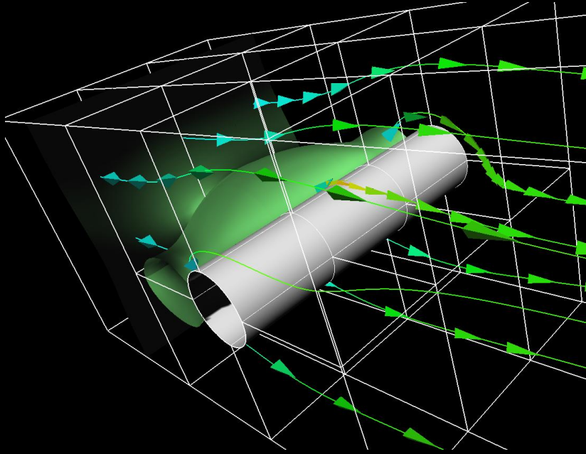
Glyphs for air flow University of Utah
