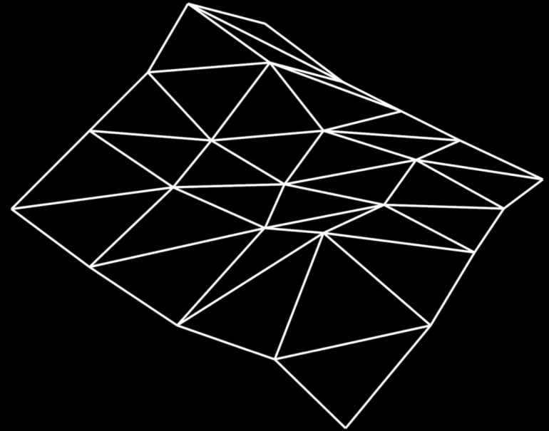
The heightfield
