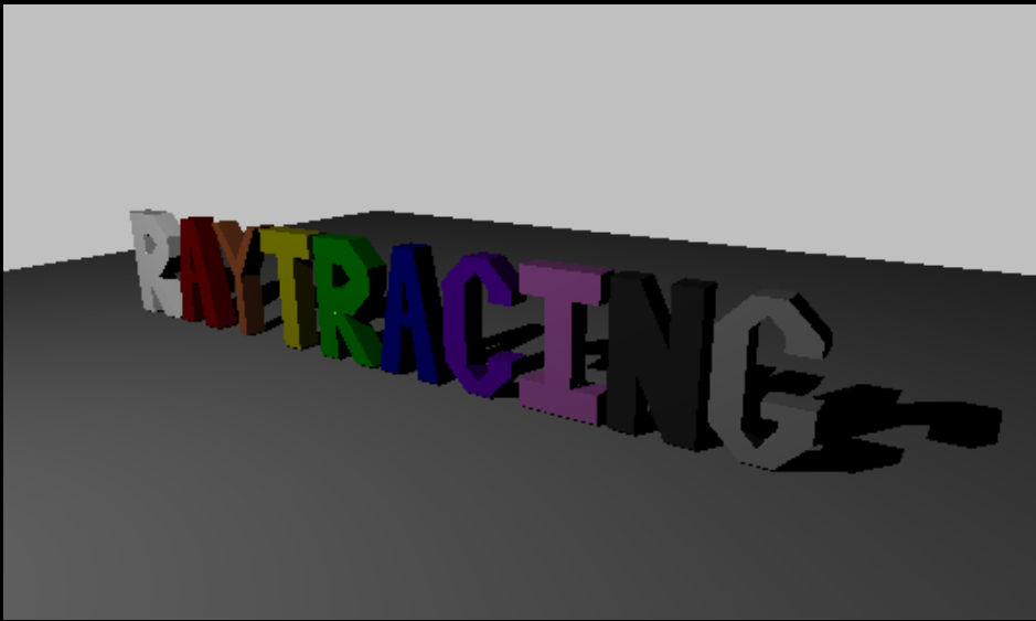
Raycasting
