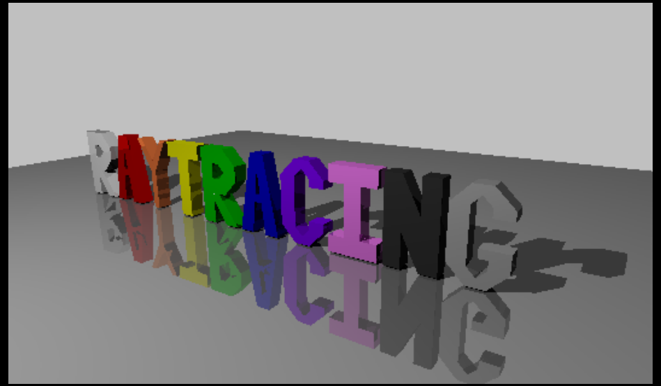
Raytracing
