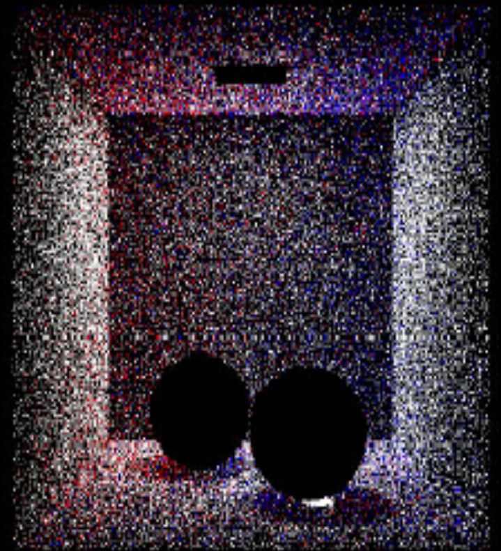
Photon Map
