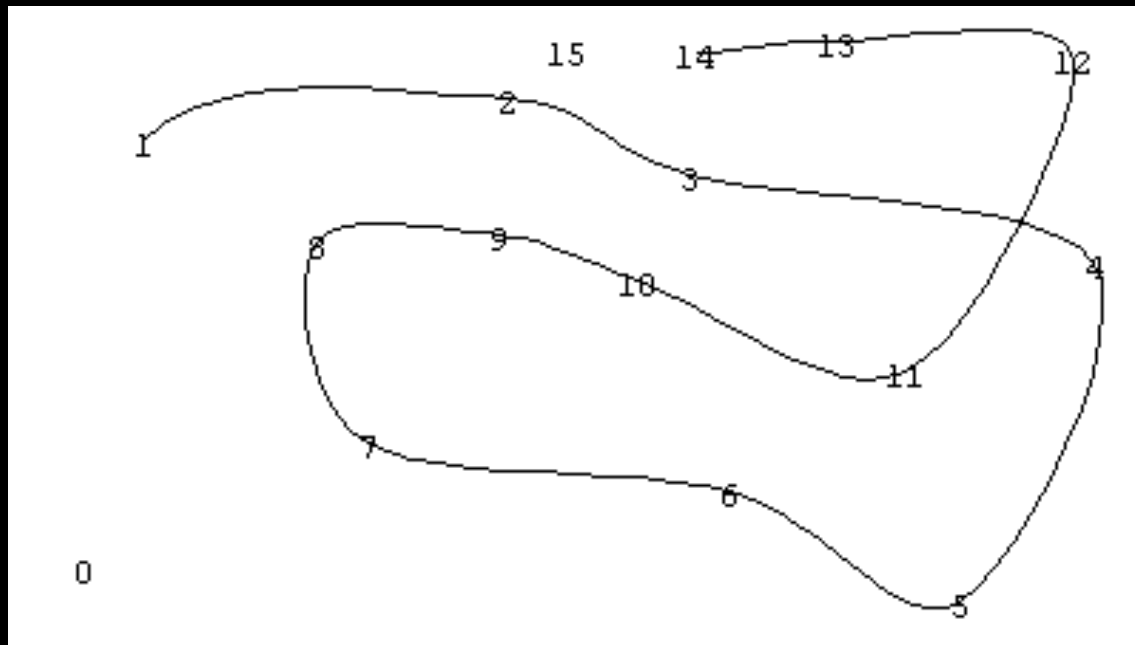
Catmull-Rom spline
