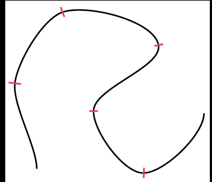
a spline
