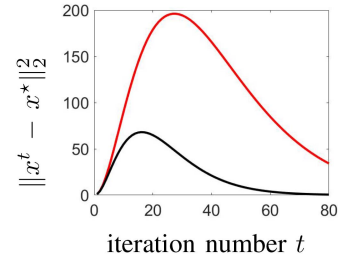
Fig. 1. Error in the optimization variable for Polyak’s heavy-ball (black) and Nesterov’s (red) algorithms with the parameters that optimize the convergence rate for a strongly convex quadratic problem with the condition number 10^3 and a unit norm initial condition with x^0 \neq x^* .
