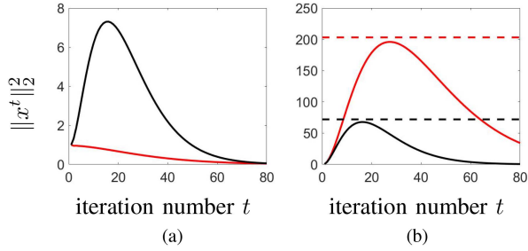
Fig. 2. Dependence of the error in the optimization variable on the iteration number for the heavy-ball (black) and Nesterov's methods (red), as well as the peak magnitudes (dashed lines) obtained in Proposition 2 for two different initial conditions with \|x^1\|_2 = \|x^0\|_2 = 1 . (a) x^1 = x^0 (b) x^1 = -x^0 .
