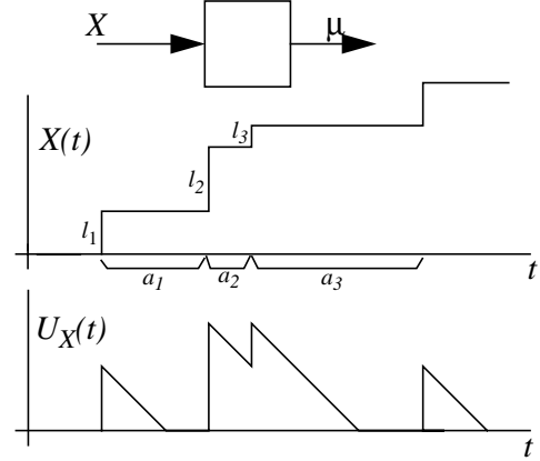
Figure 2: A work conserving */*/1 queue, and typical sample paths of accumulated and unfinished work.
