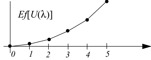
Figure 7: Convexity of unfinished work as a function of the discrete rate parameter \lambda .
