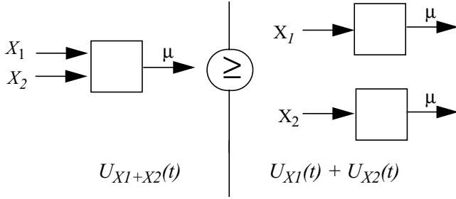
Figure 3: A queuing illustration of the non-negativity property of the blocking function.
