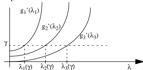
Figure 9: A sample set of \frac{d}{d\lambda_i} g_i(\lambda_i) curves.
