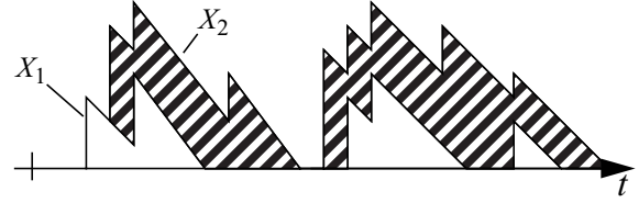
Figure 4: An example sample path of the unfinished work function U_{X_1+X_2}(t) in a system where X_1 packets have preemptive priority.
