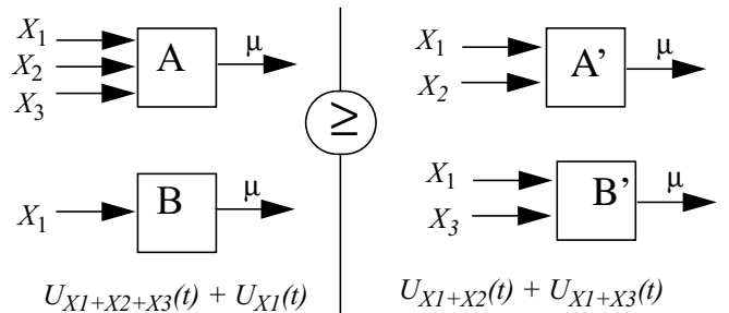
Figure 5: A queuing illustration of the monotonicity property (5) and (6).
