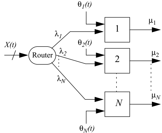
Figure 8: Multiple queues in parallel with different background processes \{\theta_i(t)\} and server rates \{\mu_i\} .
