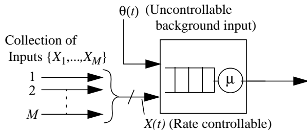
Figure 1: A work conserving queue with server linespeed \mu , a */* background input \theta(t) , and rate-controllable */* inputs X(t) = \{X_1(t), \dots, X_M(t)\} .
